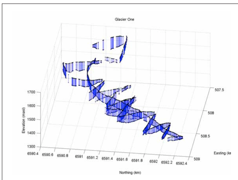
Figure 6. 3-Dimensional representation of processed radar waveform data, showing glacier surface elevation, bed elevation and ice thickness along survey transects for GL1 in Fantail Basin.
