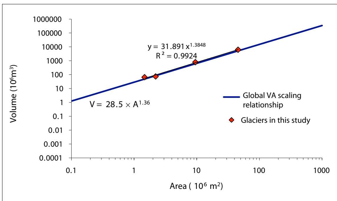
Figure 8. Comparison of glacier area and volume measurements, along with a plot of the VA scaling relationship derived from a global set of glaciers from the study of Chen and Ohmura (1990).
