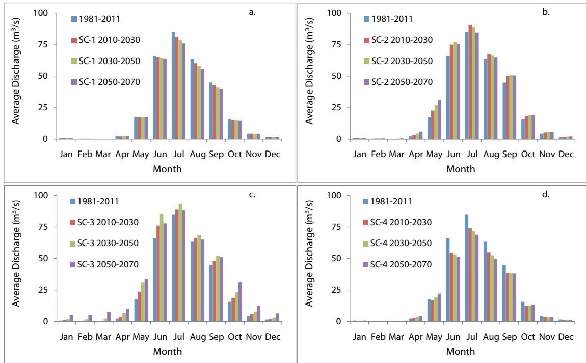
Figure 18. Monthly average discharge rate projections of Fantail River under various climate scenarios. The 1981 – 2011 simulation results are shown for comparison with contemporary hydrograph magnitude and seasonality patterns.
