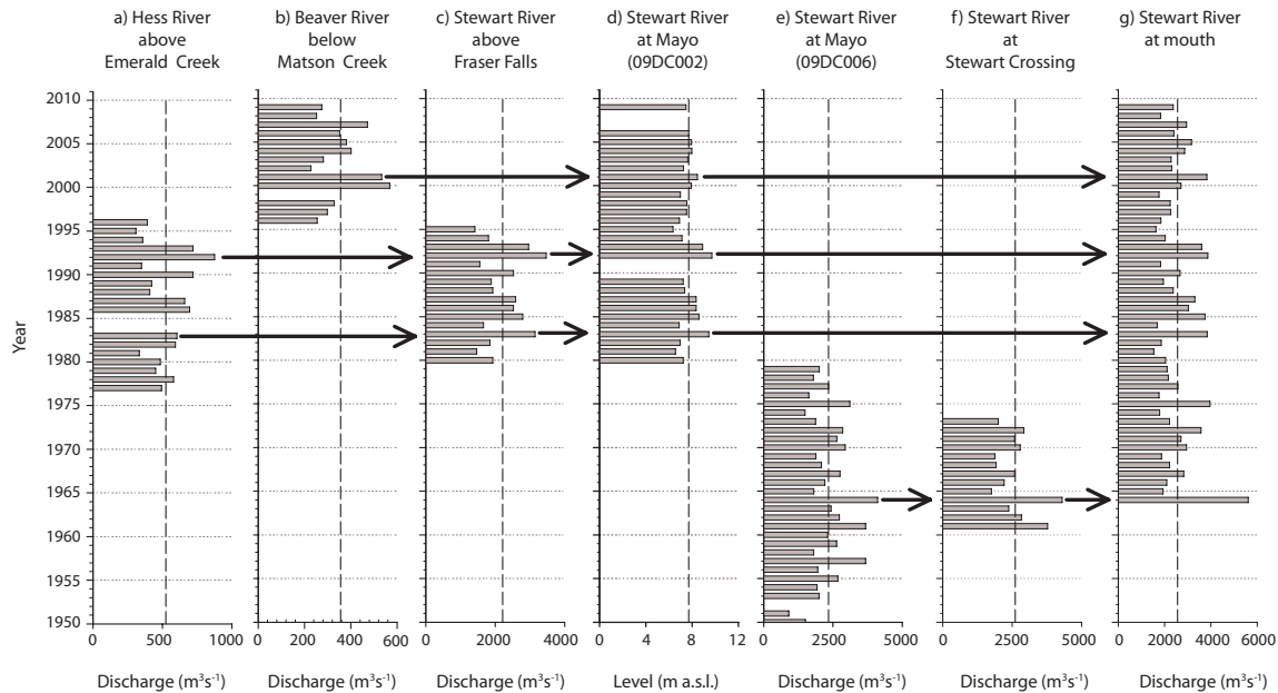
Figure 4. Peak discharge ( \text{m}^3\text{s}^{-1} ) at WSC stations ranging from the headwaters of the Stewart River (plot a) to its mouth at the Yukon River (plot g; Water Survey of Canada, 2010). Note: plot d shows level in “metres a.s.l.” rather than discharge. Vertical, long, dashed lines indicate average peak discharge for each station for its period of record. Arrows highlight events of above-average peak discharge (or level) that are evident in all existing records, demonstrating how peaks in headwater discharge propagate downstream.
