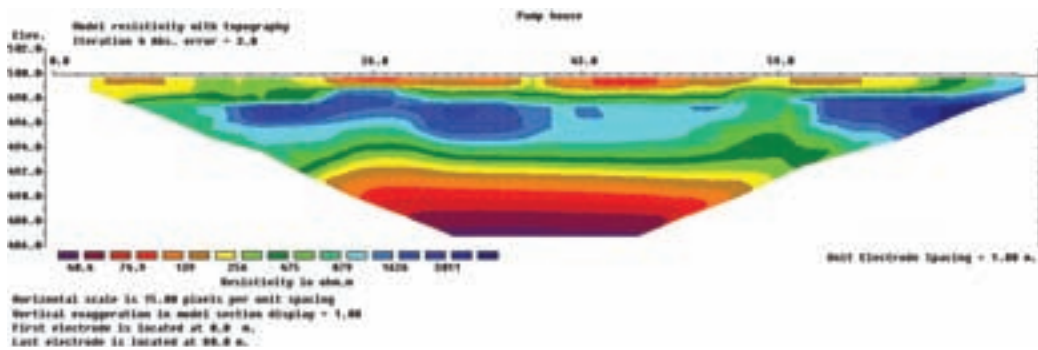
Figure 28. Resistivity profile near the pump house, Mayo.
